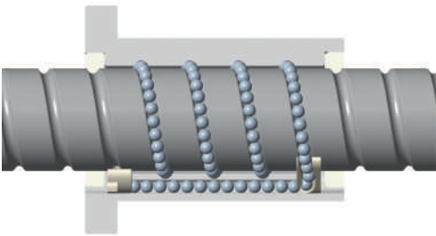
U-type recirculation system
