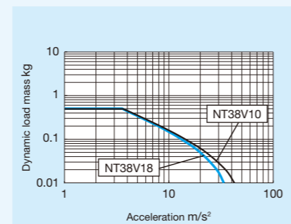
Fig. 5 Dynamic load mass of NT38V
