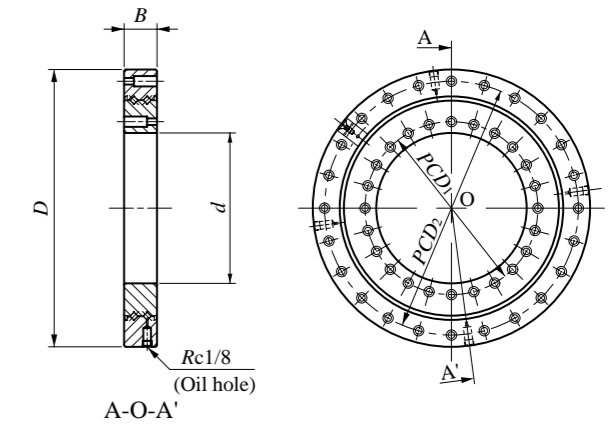
Fig. 5 Manufacturing example
